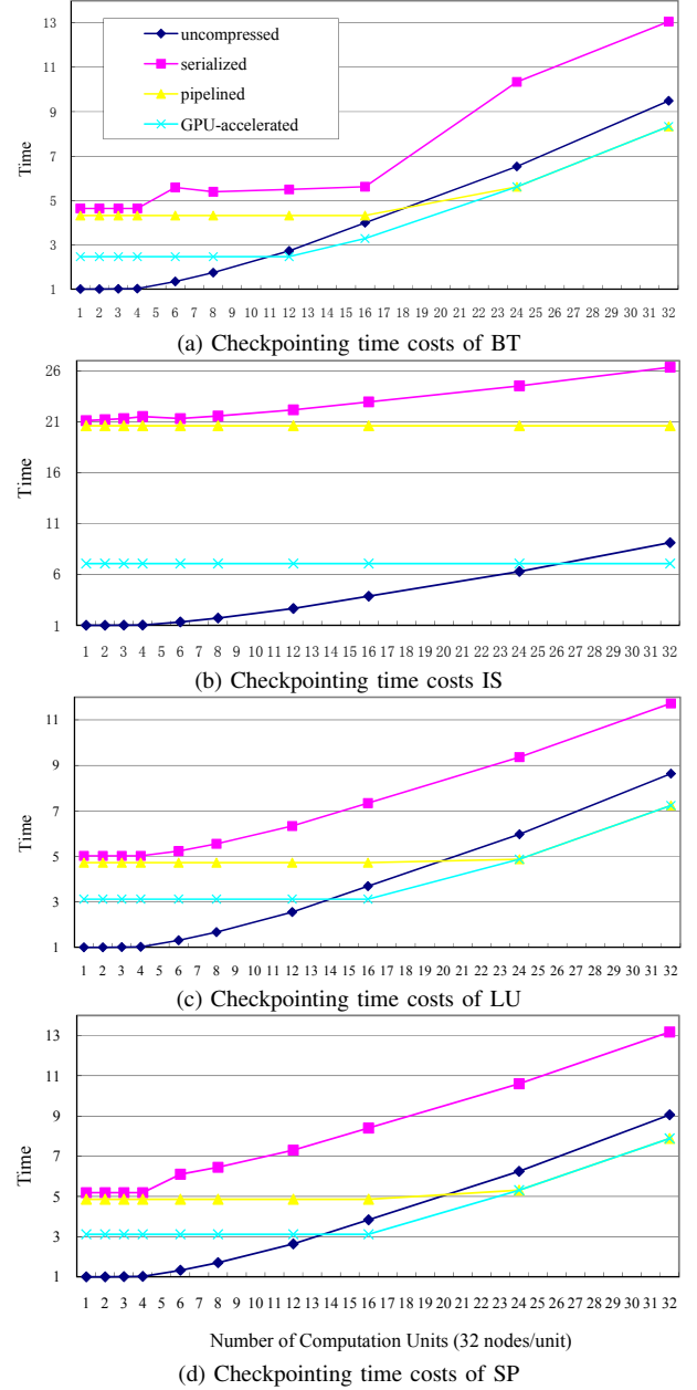
Figure 12. Relationship between Time Costs and System Scales
