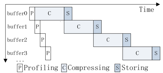
Figure 7. Pipelining of Compression Checkpointing
