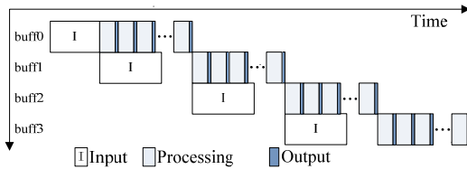
Figure 8. Pipeline of GPU-Accelerated String Matching
